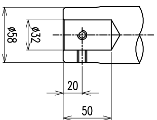
SHANK HOLE
