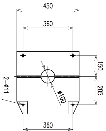
BOLSTER DIMENSION
